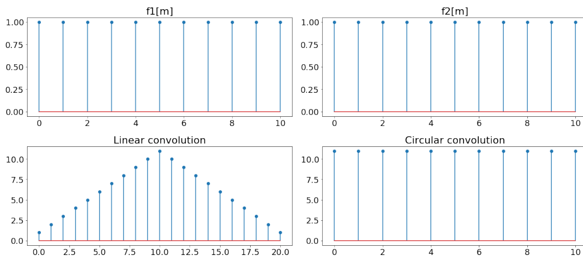
Figure 13.1: Difference between linear and circular convolution of two finite discrete sequences. The linear convolution of two length- N sequences leads to a length- (2N-1) sequence, which resembles the continuous convolution we have covered earlier in this course. The circular convolution two length- N sequences leads to a length- N sequence, as described in this lecture.
