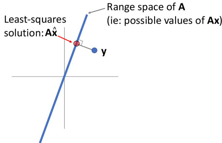
Figure 21.1: Geometric interpretation of the solution to a linear least-squares problem.
