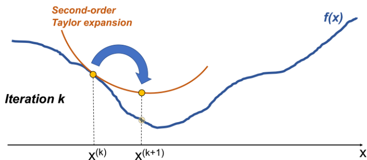
Figure 28.1: Pictorial depiction of the Newton method.
